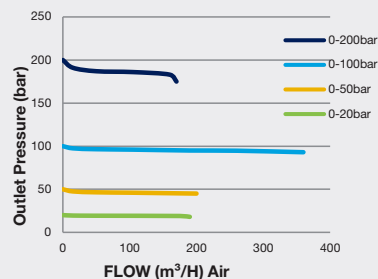
200 bar Inlet Pressure @ 21° C
